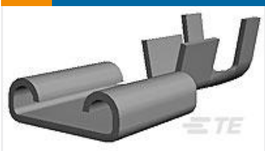
TE Part #62998-2 250 FSATON REC 10-8 AWG TPBR
