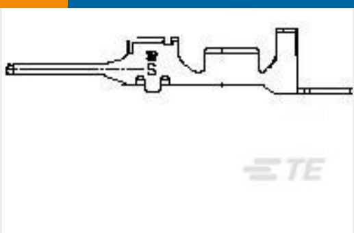
TE Part #1-2040016-2 DYNAMIC D4200 TAB CONT S LONG
