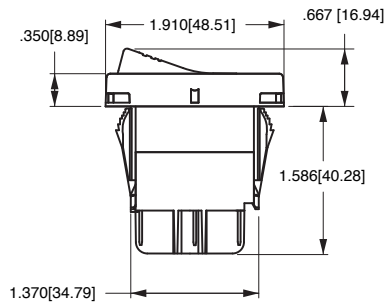
8 TERMINAL BASE W/BARRIERS
