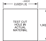
MOUNTING PANEL OPENING (2) UNITS
