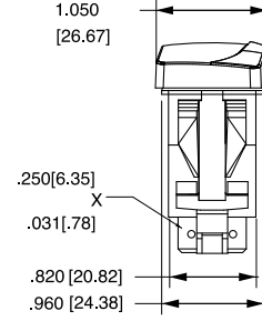
10 TERMINAL BASE W/O BARRIERS
