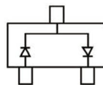
Equivalent Circuit
