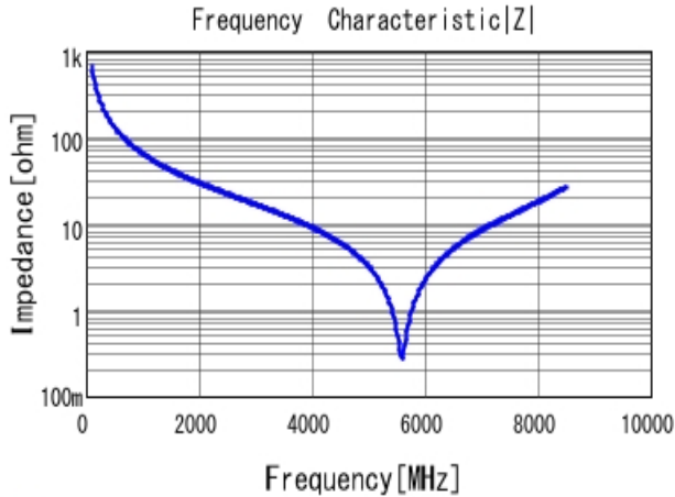
■ GJM1555C1H2R4BB01 |Z| DC0V, 25degC
