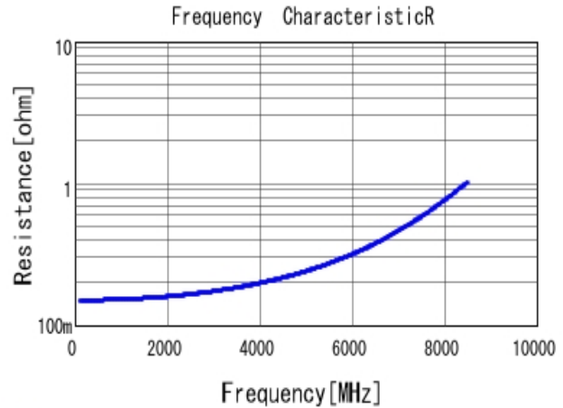
■ GJM1555C1H2R4BB01 R DC0V, 25degC
