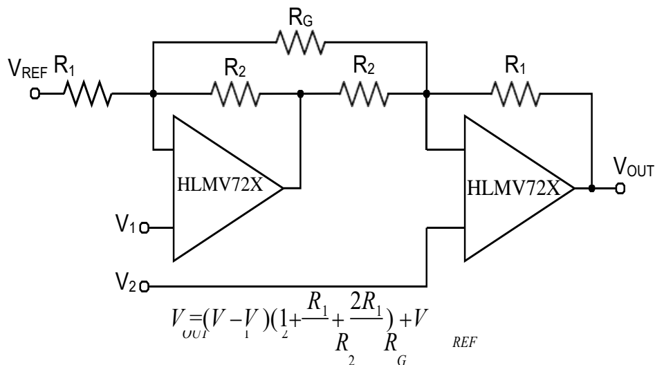
Fig. 17 Instrumentation Amplifier
