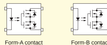
Form-A contact Form-B contact
