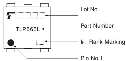
(b) 5 pin DIP6 Package (TLP665L)
