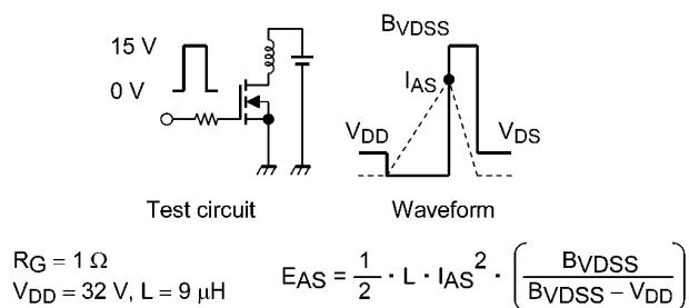
Fig. 9.16 Test Circuit/Waveform
