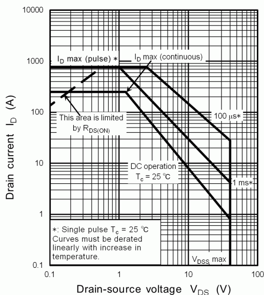
Fig. 9.14 Safe Operating Area (Guaranteed Maximum)
