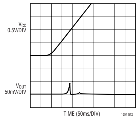
V_{OUT} Glitch at Power-Up
