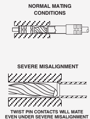
Figure 2 - Illustrates the Twist Pin features, as well as mating & severe misalignment conditions.
