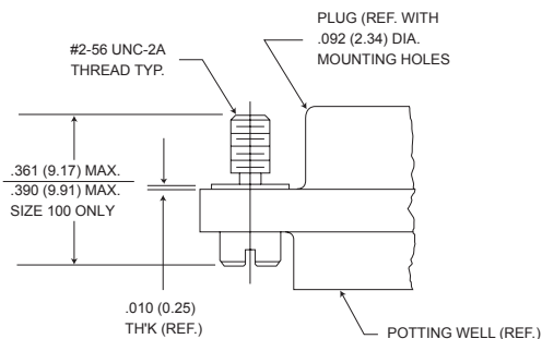
Figure 1. Jackscrew - Low profile Slotted Head Size 9-69 Size 100*
