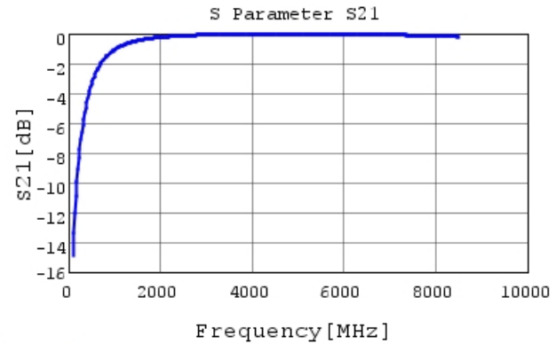
GJM1555C1H2R9CB01 S21 DCOV, 25degC
