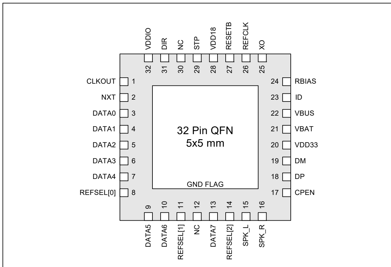
FIGURE 2-1: USB3340 PIN LOCATIONS - TOP VIEW
