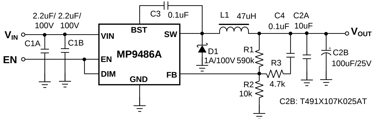
Figure 5: V_{IN}=15\sim95V , V_{OUT}=12V , I_{OUT}=1A
