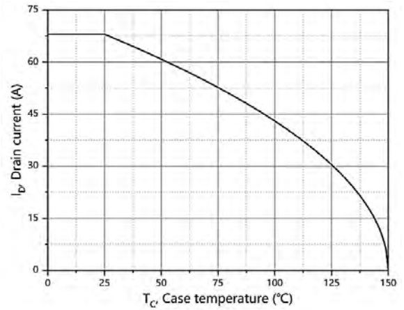
Figure 10. Drain current
