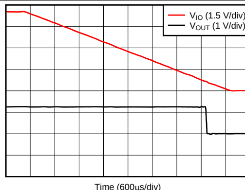
Figure 44. V_{IO} Power-Down
