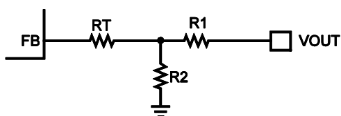
FIGURE 6. T-Type Network
