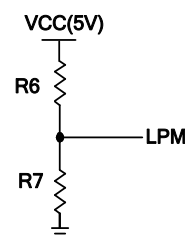
FIGURE 7. LPM Network
