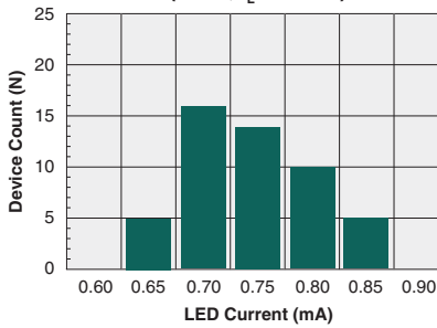
Typical I_F for Switch Dropout (N=50, I_L=120\text{mA} )
