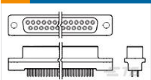
TE Part #5745080-4 HD-20 RCPT 50P VERT FFSCRLK
