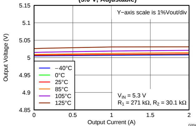
LOAD REGULATION (5.0 V, Adjustable)
