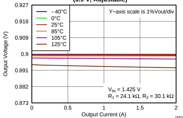
LOAD REGULATION (0.9 V, Adjustable)
