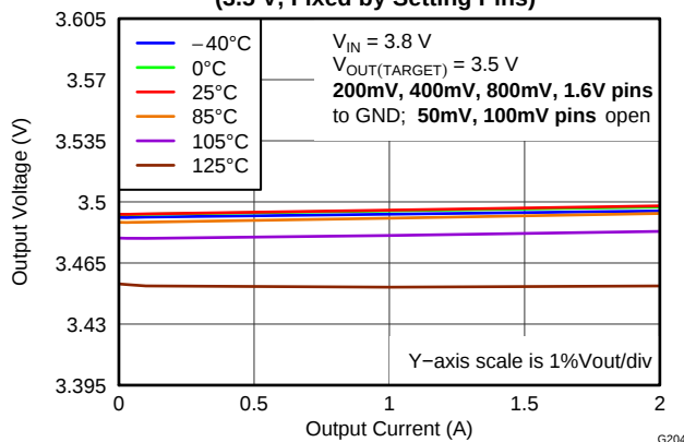
LOAD REGULATION (3.5 V, Fixed by Setting Pins)
