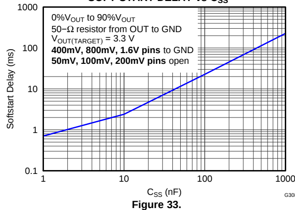
SOFT-START DELAY vs C_{SS}
