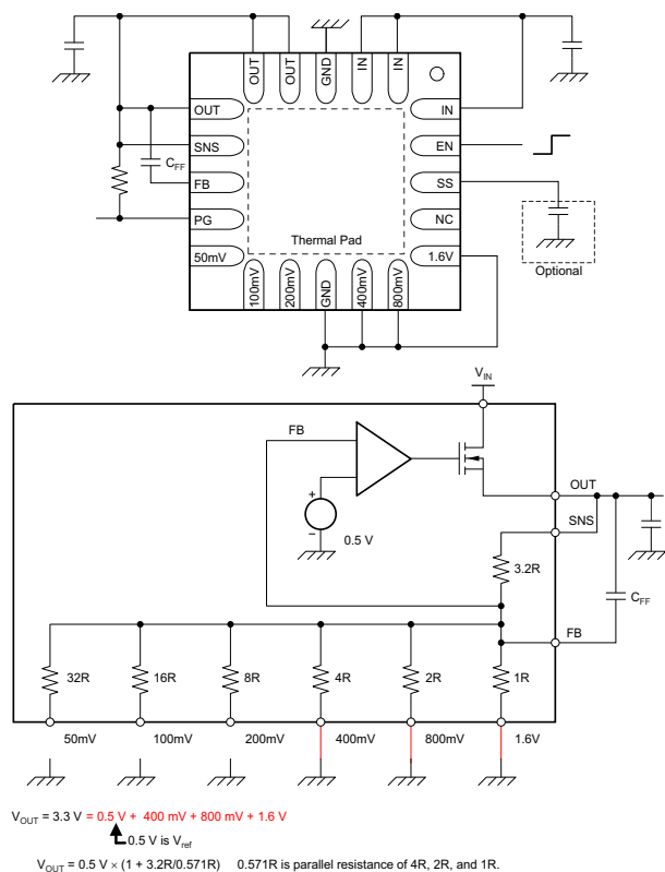
Figure 38. 3.3-V Configuration
