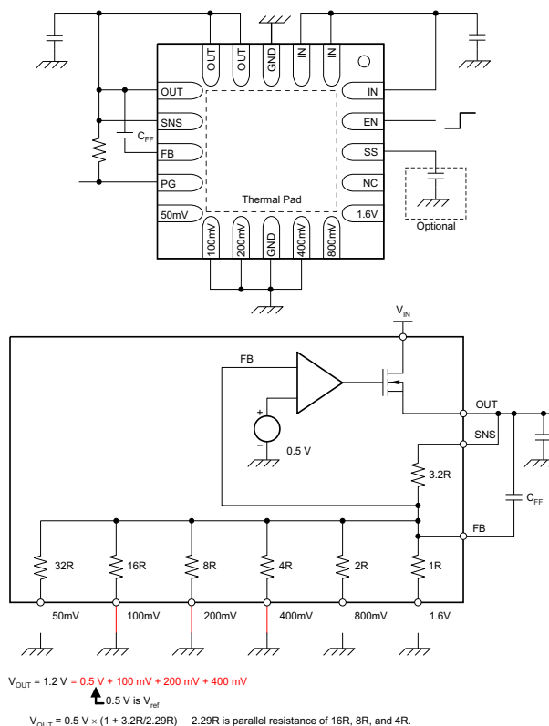
Figure 35. 1.2-V Configuration
