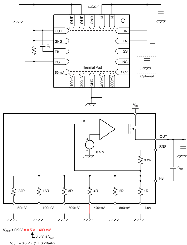
Figure 34. 0.9-V Configuration
