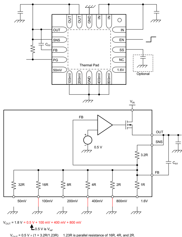
Figure 36. 1.8-V Configuration
