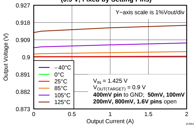
LOAD REGULATION (0.9 V, Fixed by Setting Pins)
