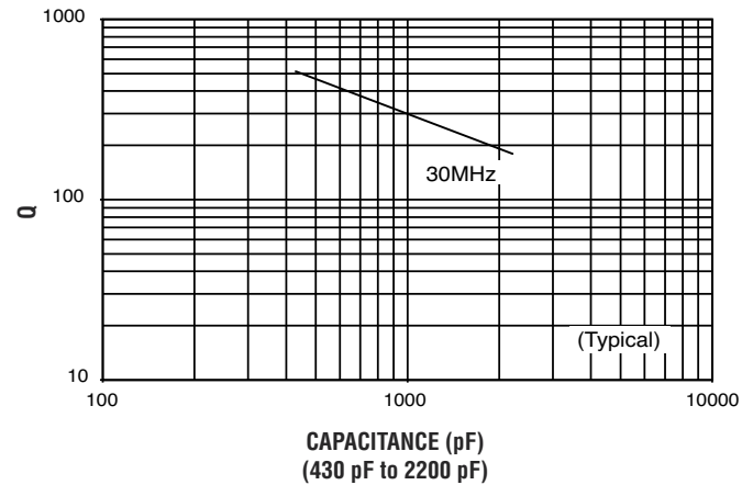
Q VS. CAPACITANCE ATC SERIES 700, CASE E
