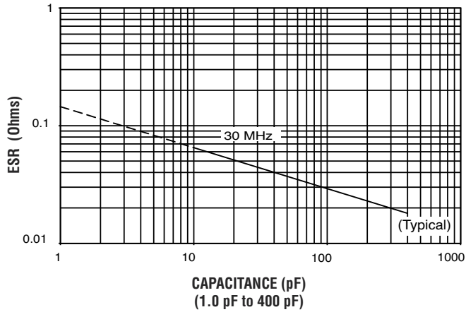
ESR VS. CAPACITANCE ATC SERIES 700, CASE E
