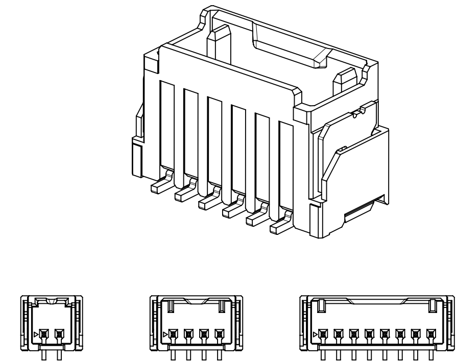
VIEW OF 2-3 CIRCUIT VIEW OF 4-6 CIRCUIT VIEW OF 7-8 CIRCUIT
