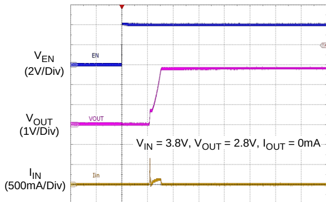
Inrush Current
