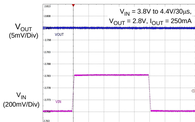
Line Transient
