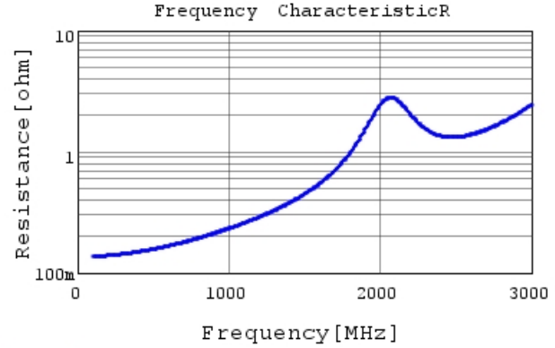
GCM31A5C2J680FX01 R DC0V, 25degC
