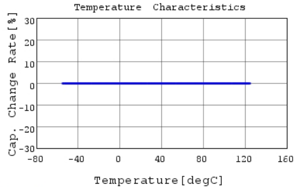
GCM31A5C2J680FX01 C-Temp. capchange, DC0V, 1
