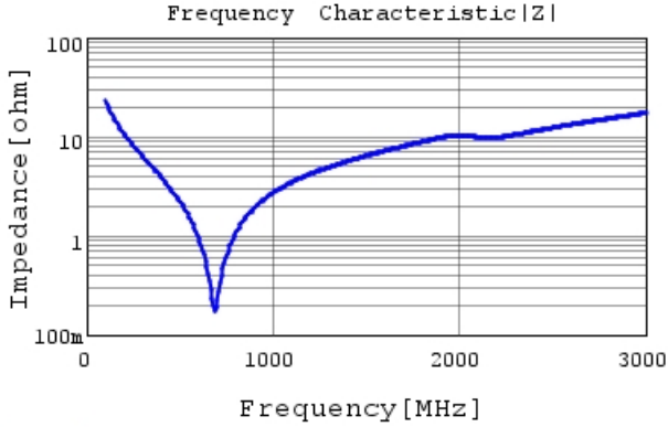
GCM31A5C2J680FX01 |Z| DC0V, 25degC
