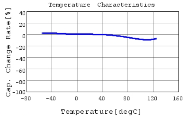
GCH155R72A222KE01 C-Temp. capchange, DC0.0V,
