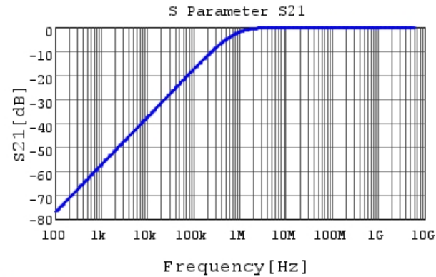
GCH155R72A222KE01 S21 DC0V, 25degC
