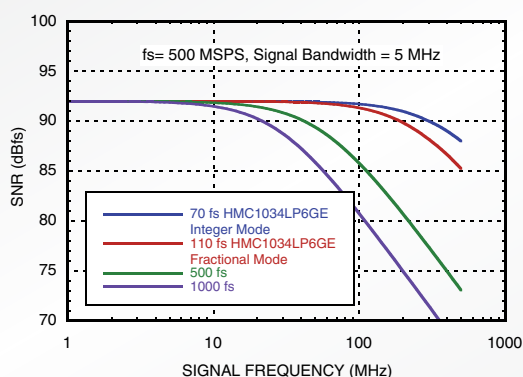
ADC SNR vs. Clock Jitter and Input Frequency
