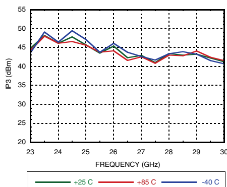
Input IP3 vs. Temperature @ 10 dBm/tone
