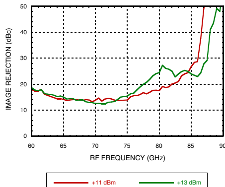
Image Rejection, USB vs. LO Power
