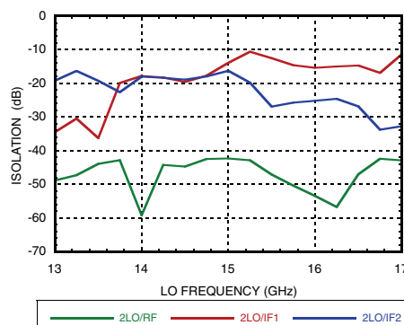
2LO Isolation
