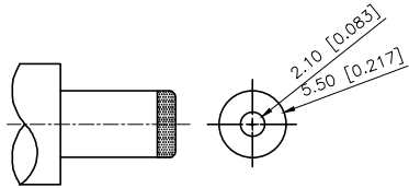
MATING PLUG Jack Insertion Depth: 9.5 mm
