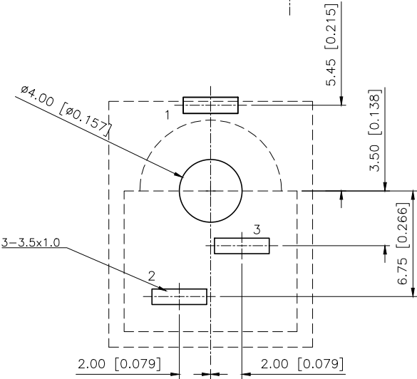
PCBLAYOUT FRONT VIEW
