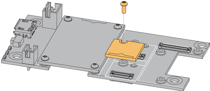
Figure 2: RAK12003 WisBlock Infrared Temperature Sensor Mounting
