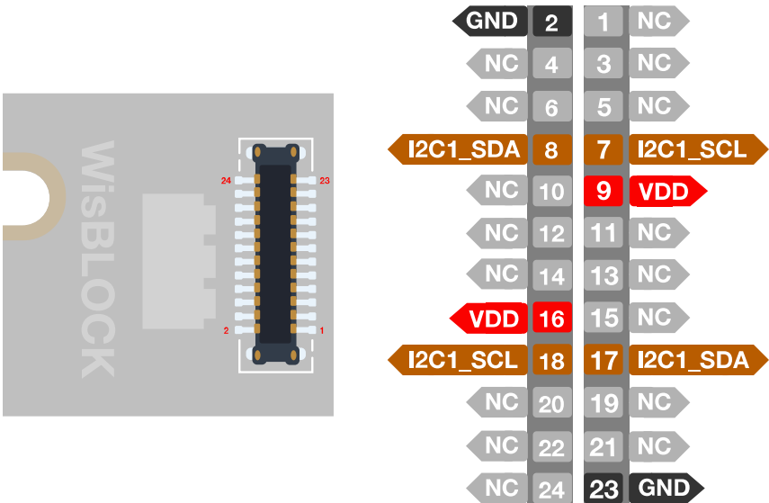
Figure 4: RAK12003 WisBlock Infrared Temperature Sensor connector pinout
