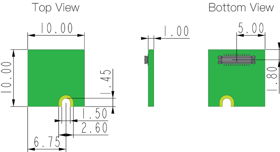
Figure 5: RAK12003 WisBlock Infrared Temperature Sensor Mechanic Drawing
