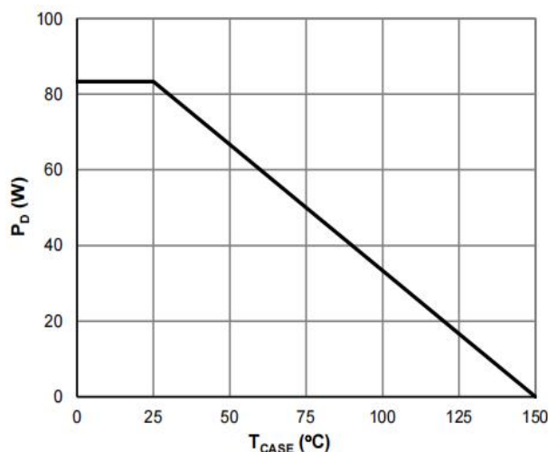
Figure 10: Power De-rating
