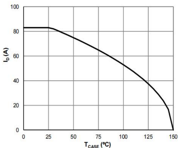
Figure 9: Current De-rating
