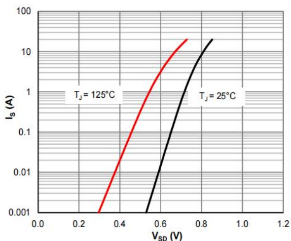
Figure 7: Body-Diode Characteristics
