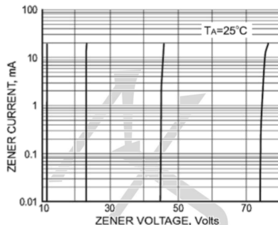
ZENER BREAKDOWN CHARACTERISTICS
