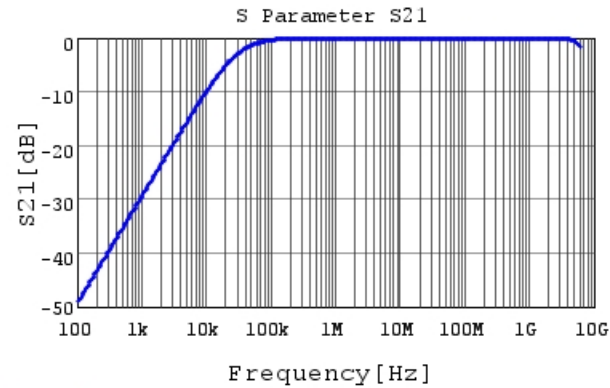
GCJ188R71H563KA12 S21 DC0V, 25degC
