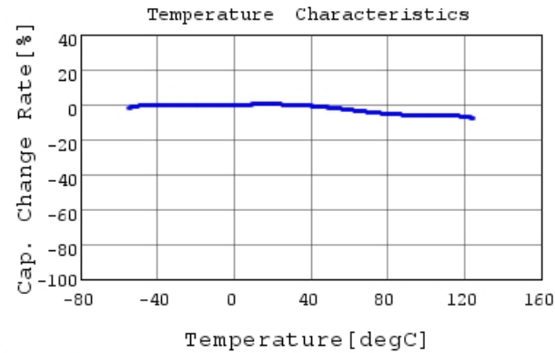
GCJ188R71H563KA12 C-Temp. capchange, DC0.0V,
