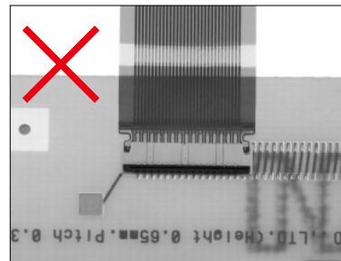
Partial insertion
