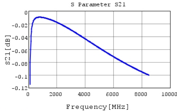
GRM0115C1E101GE01 S21 DCOV, 25degC
