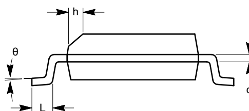
END VIEW
