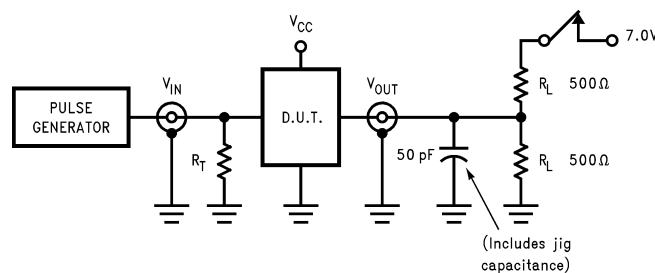
Figure 6. Test Circuit For TRI-STATE Outputs On A Side
