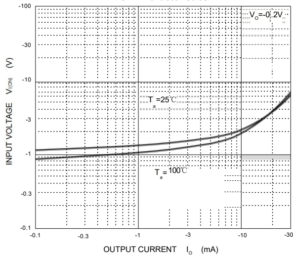
ON Characteristics
