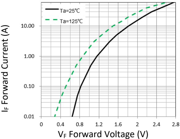
Figure 1. Forward Characteristic(typ.)
