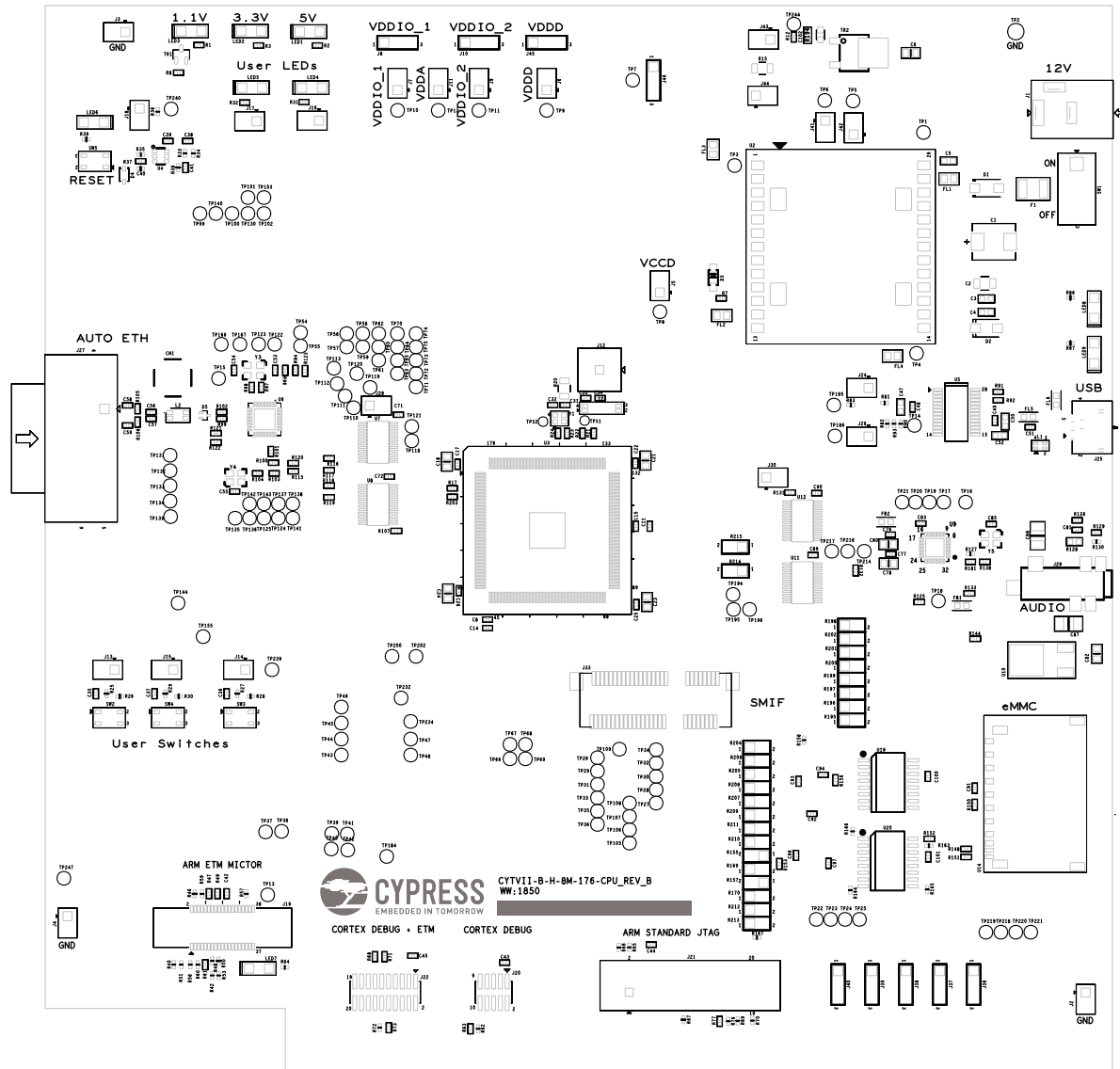
Figure B-1. Component Assembly (Top)
