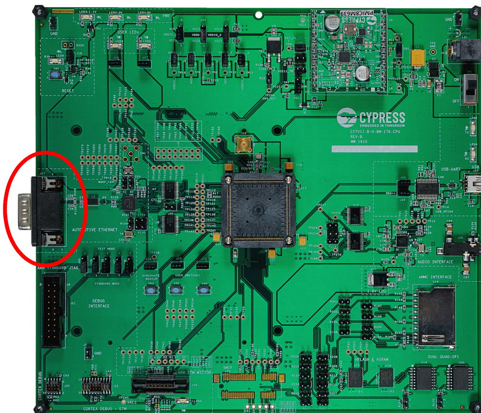
Figure 2-6. Ethernet Connector
