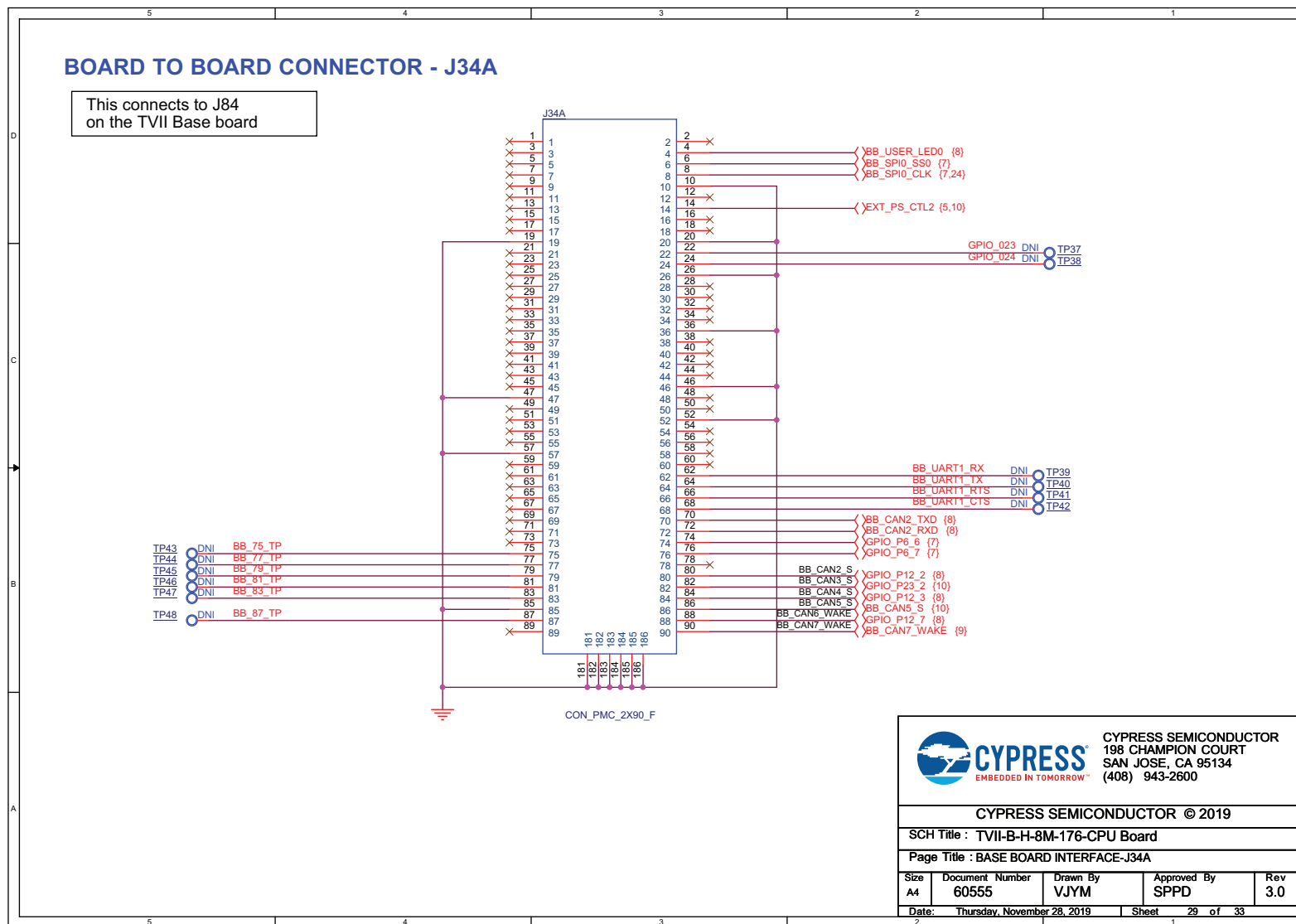
Figure A-28. Schematic (28/31)
