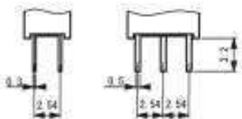
Terminal style of c (Style : PC Terminal)
