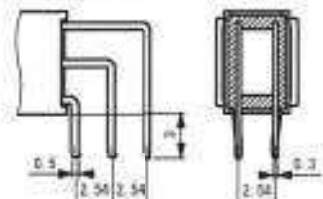
Terminal style of C6 (Style : V/M Terminal)
