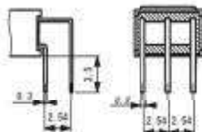
Terminal style of C4 (Style : R/A Terminal)
