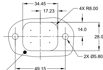
RECOMMENDED PANEL CUTOUT TYPE 2
