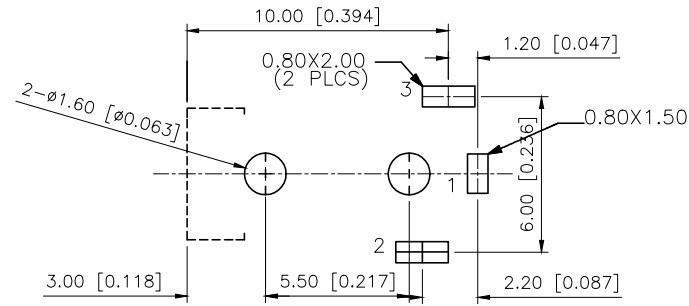
PCB LAYOUT
