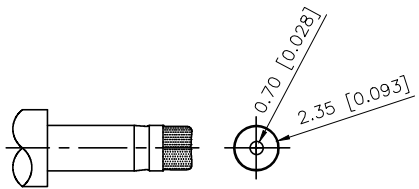
MATING PLUG Jack Insertion Depth: 8.0 mm
