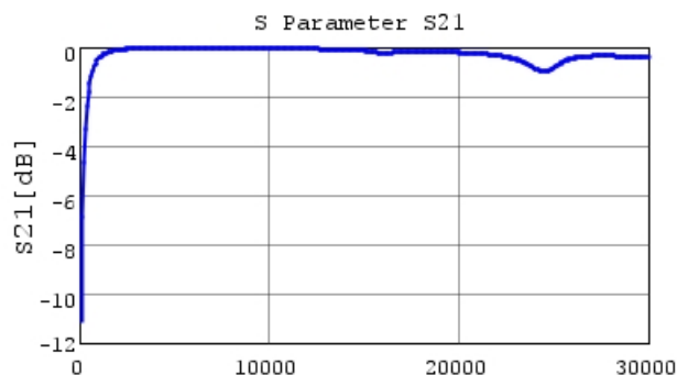
■ GJM0225C1C4R6BB01 S21 DCOV, 25degC
