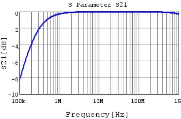
RHEL82A682K0DBH03A S21 DCOV, 25degC
