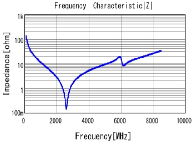
■ GJM1555C1H120GB01 |Z| DC0V, 25degC
