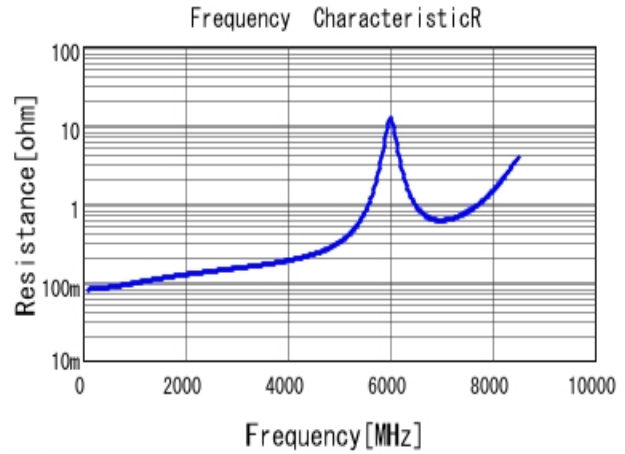
■ GJM1555C1H120GB01 R DC0V, 25degC
