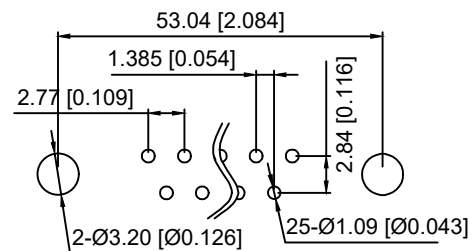
PCB LAYOUT
