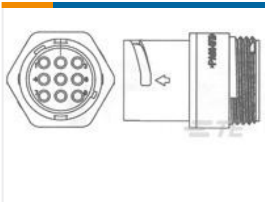
TE Part #1445829-1 REC,11-5,FRE HNG,SM INS,STD KE
