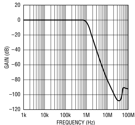
Figure 5. Frequency Response of Filter
