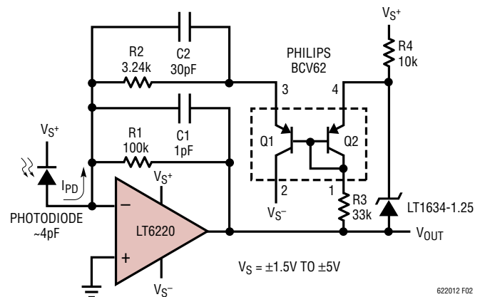
Figure 2. Stepped-Gain Photodiode Amplifier
