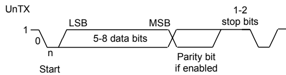
Figure 11-2. UART Character Frame
