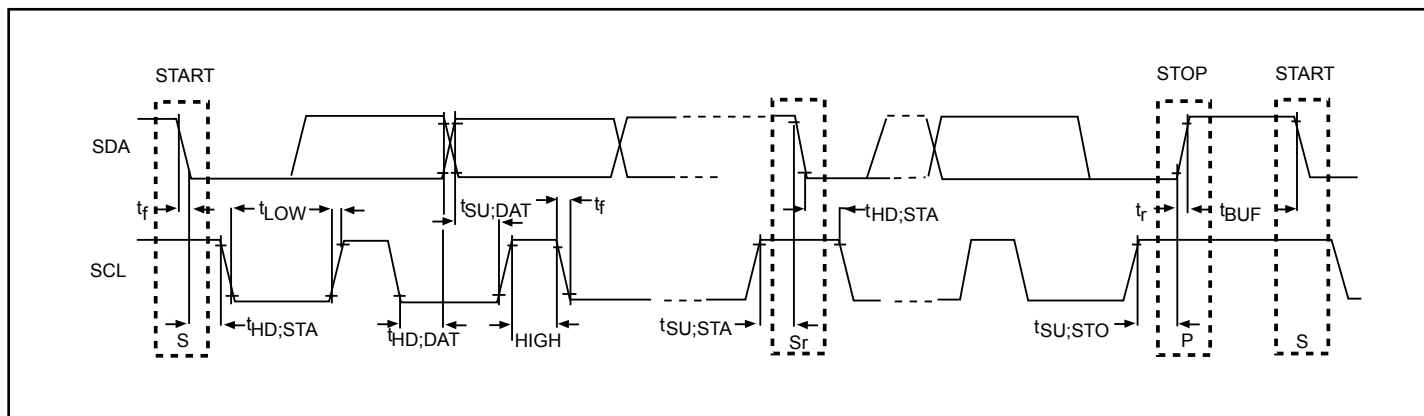
I²C Timing
