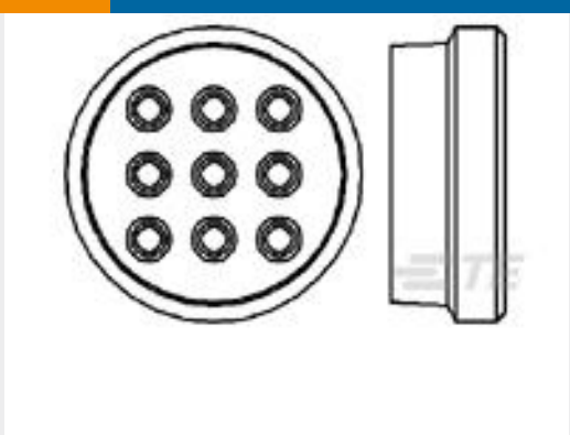
TE Part #213926-1 CPC SEAL ASSY KIT,RH,SR 1,13-9
