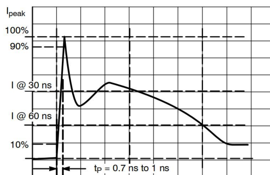
Fig2. IEC61000-4-2 Waveform
